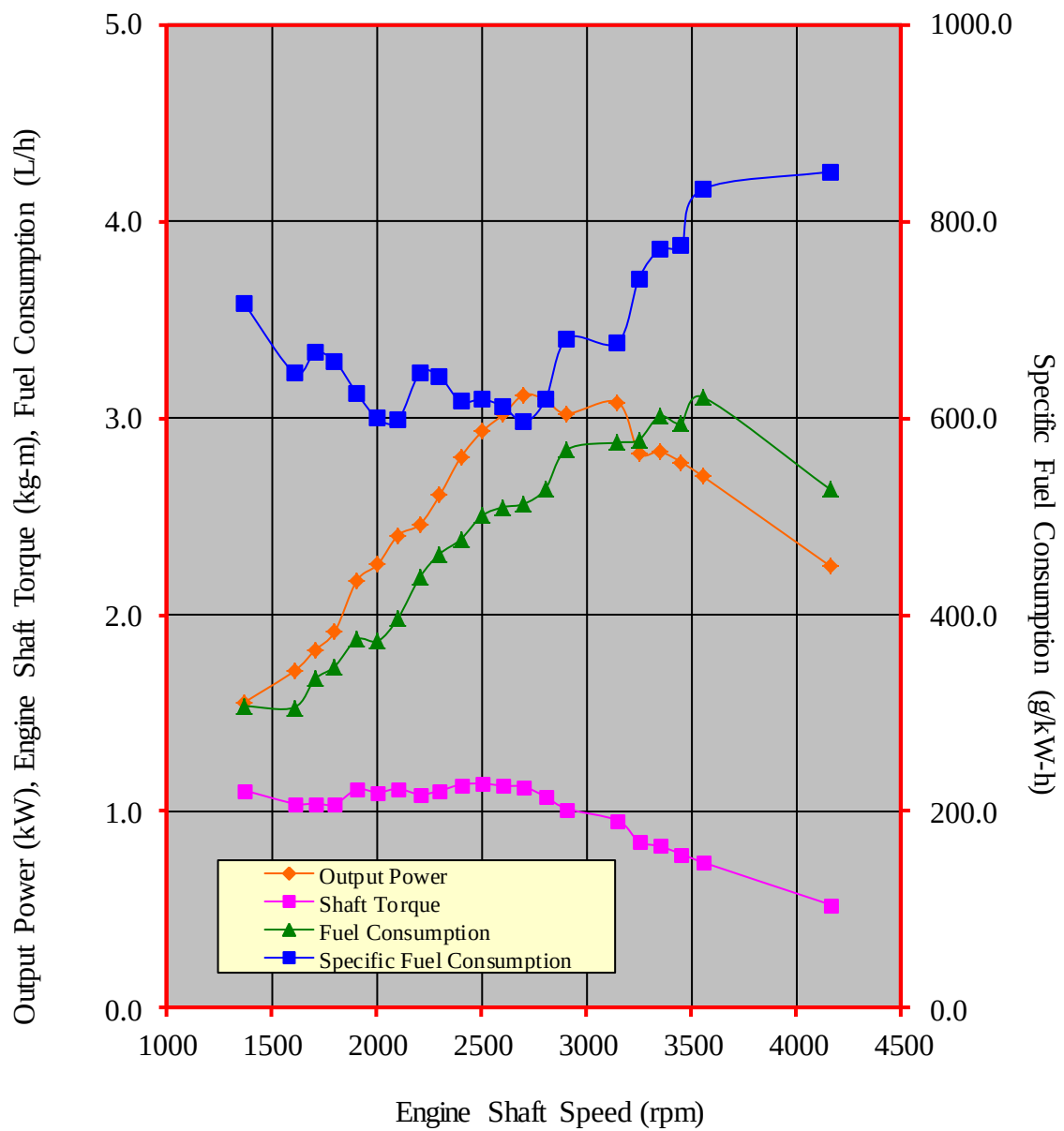
Figure 3. Performance characteristic curves of the MASTER MARINE ESE 173F diesel engine
