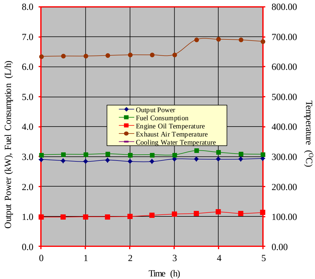
Figure 4. Performance characteristic curves during the continuous running test of MASTER MARINE ESE 173F diesel engine
